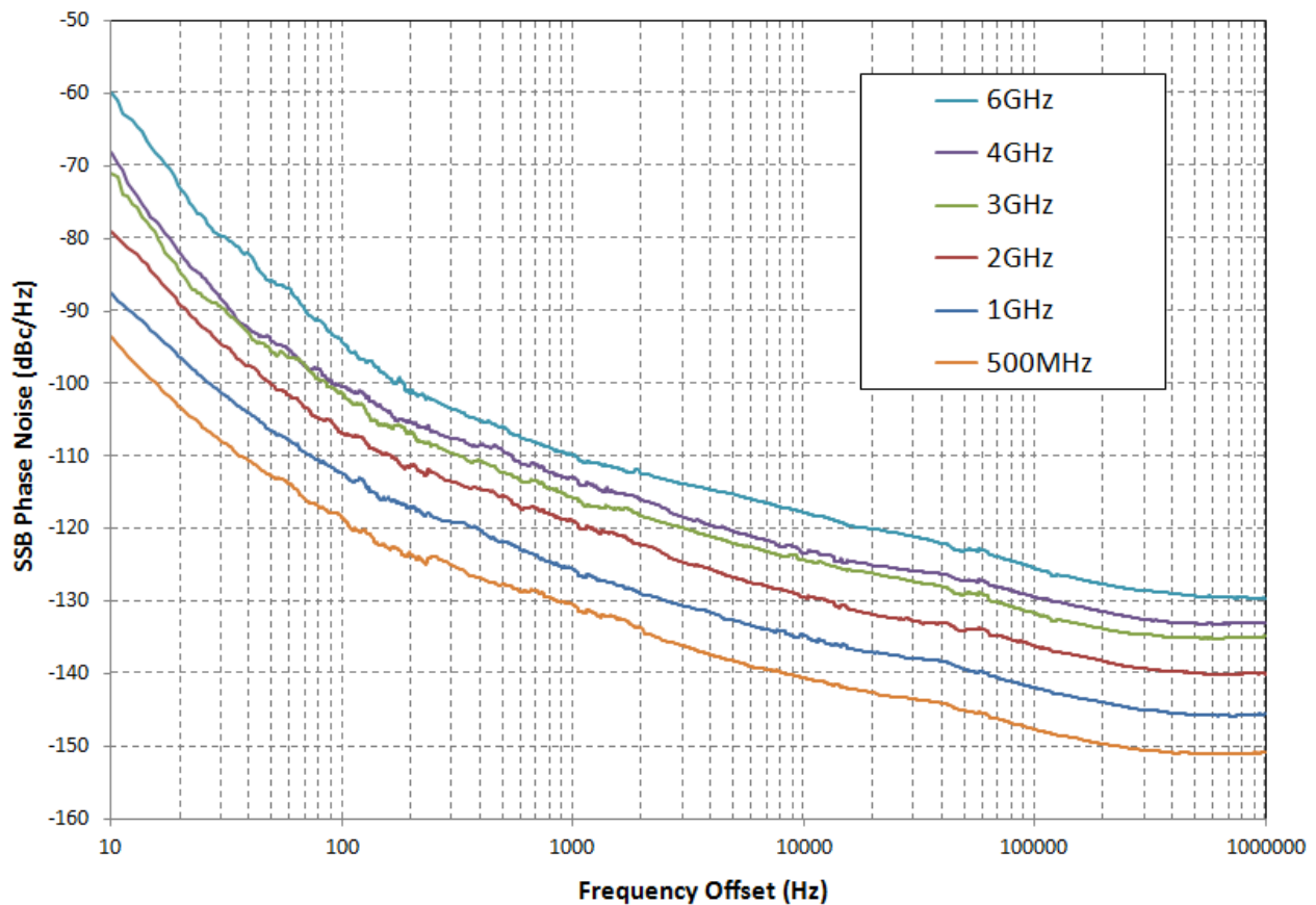
Figure 5: Channel SSB Phase Noise (P OUT =+10dBm)
