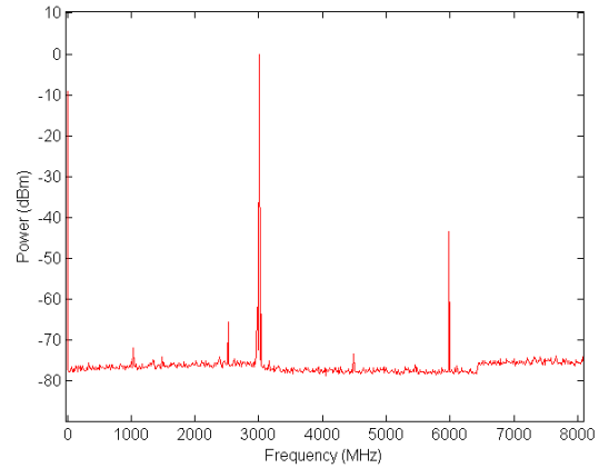
Figure 10b: 3GHz Broad Band Spectrum
