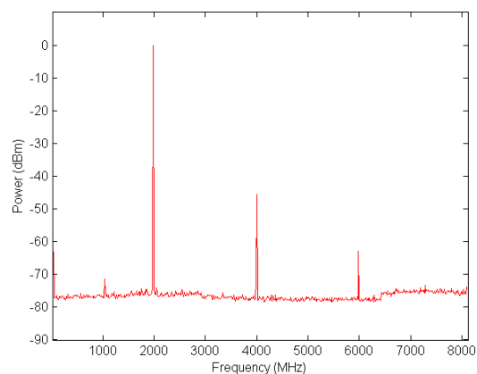
Figure 9b: 2GHz Broad Band Spectrum
