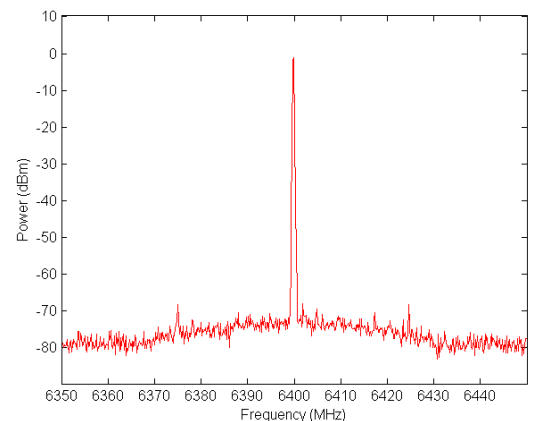
Figure 12a: 6.5GHz Narrow Band Spectrum
