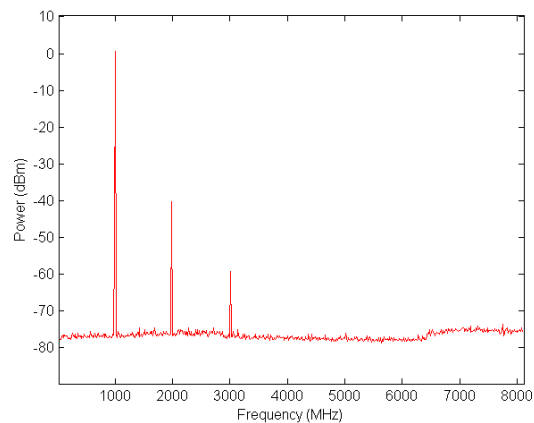
Figure 8b: 1GHz Broad Band Spectrum
