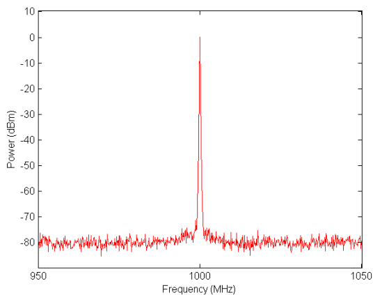
Figure 8a: 1GHz Narrow Band Spectrum
