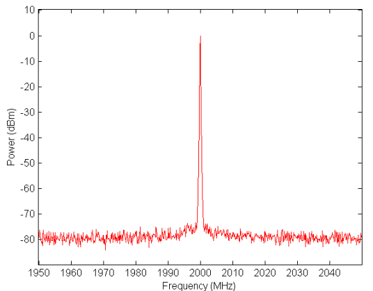
Figure 9a: 2GHz Narrow Band Spectrum
