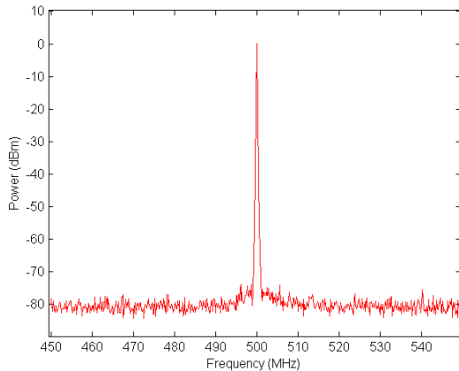
Figure 7a: 500MHz Narrow Band Spectrum
