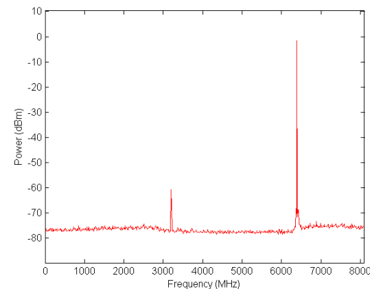
Figure 12b: 6.5GHz Broad Band Spectrum
