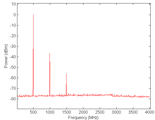
Figure 7b: 500MHz Broad Band Spectrum
