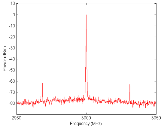
Figure 10a: 3GHz Narrow Band Spectrum
