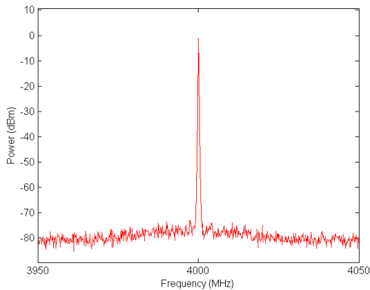
Figure 11a: 4GHz Narrow Band Spectrum
