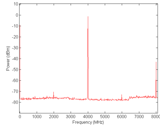
Figure 11b: 4GHz Broad Band Spectrum
